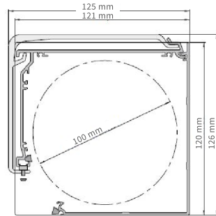
Closed Square Cassette
