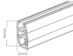
Aluminum Flat heavy duty 35x15mm
