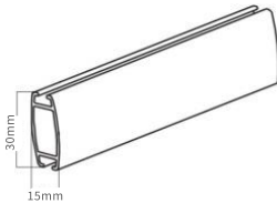
Aluminum Flat (fabric dressed) 15x30mm
