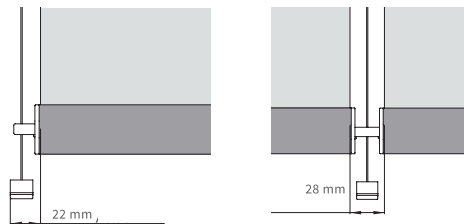
Wire side guides
