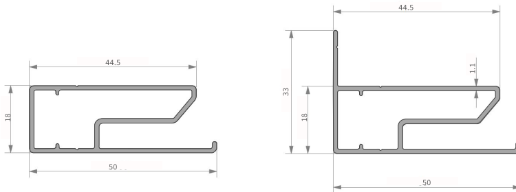
Wire side guides
